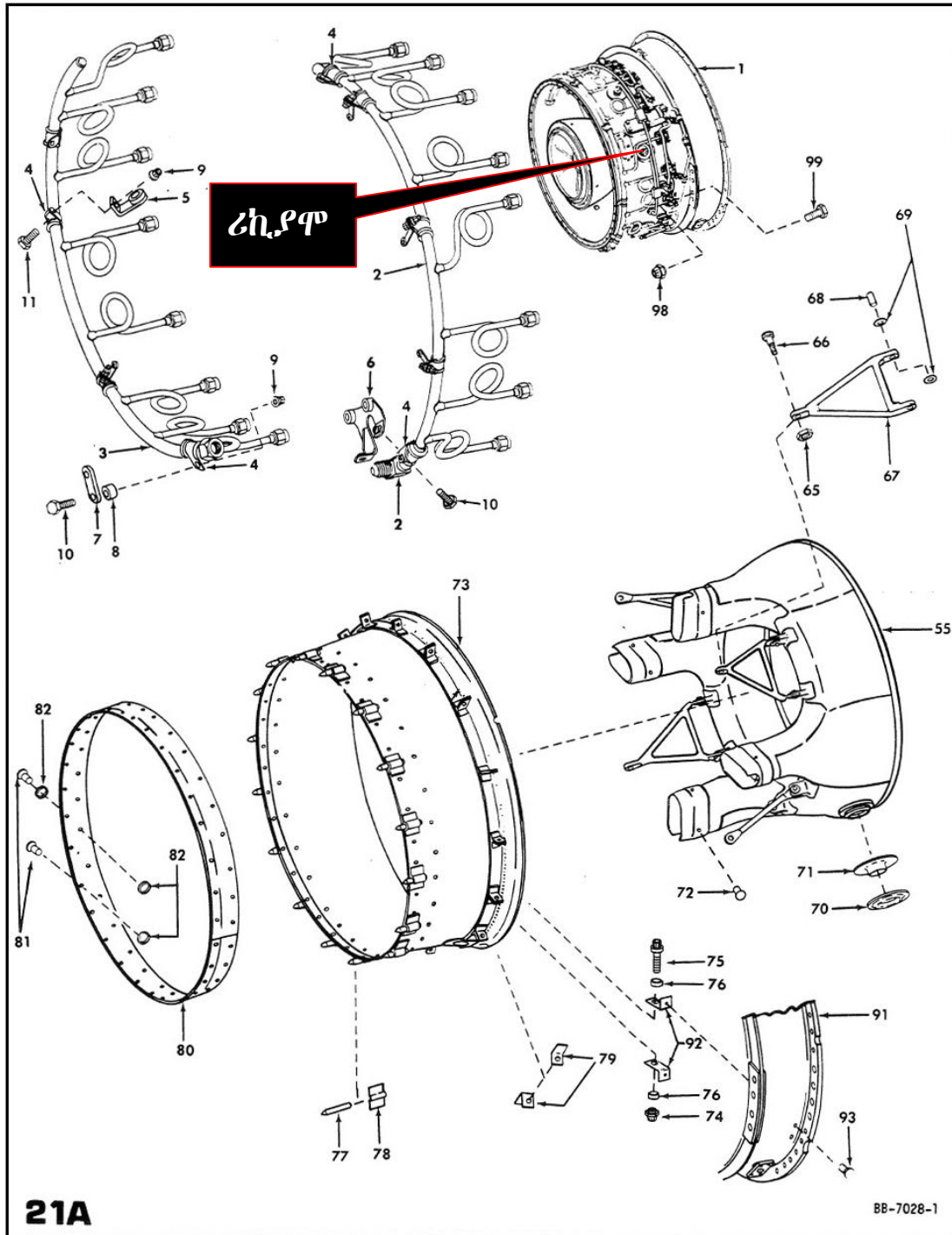
FIGURE 21A. AFTERBURNER DIFFUSER ASSEMBLY (6009T20)
